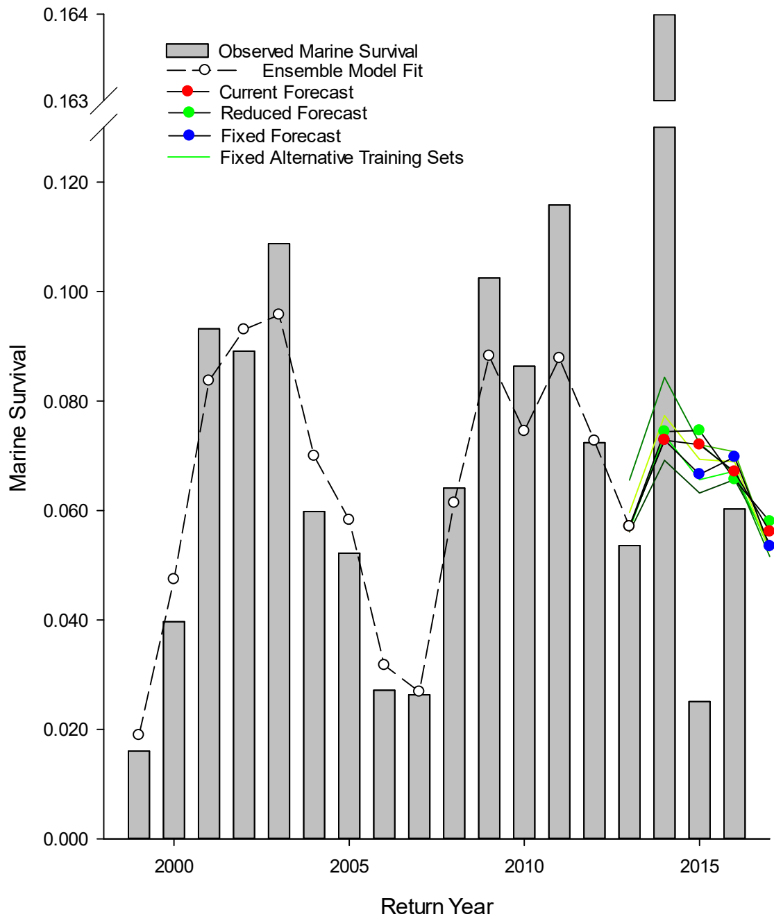
Figure 3. Observed marine survival with model fits and forecasts using the proposed methods from 2014-2017. The green lines without points show forecasts generated from fixed models with training datasets of varying length, from 1998-2010 to 1998-2014.
