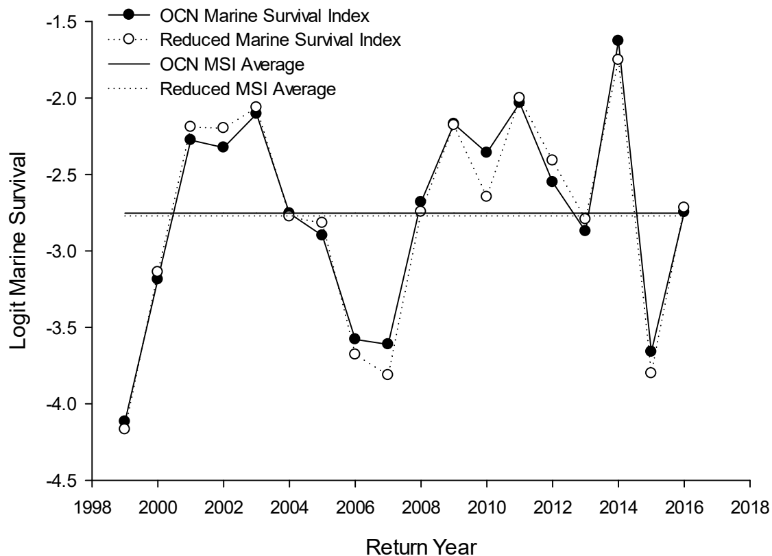
Figure 2. Time series comparison of the OCN and reduced marine survival indexes.
