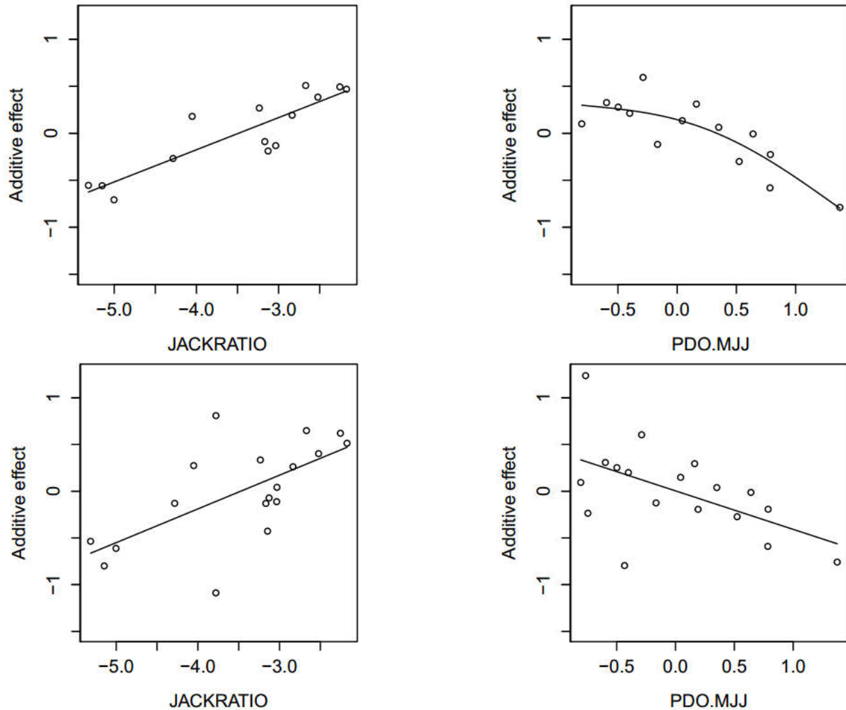
Figure 4. Partial regression plots for the 2013 revision model fit (top) and latest model fit (bottom) for the Mill Creek Yaquina LCM jack/smolt ratio and PDO May-June-July four year moving average indicators.
